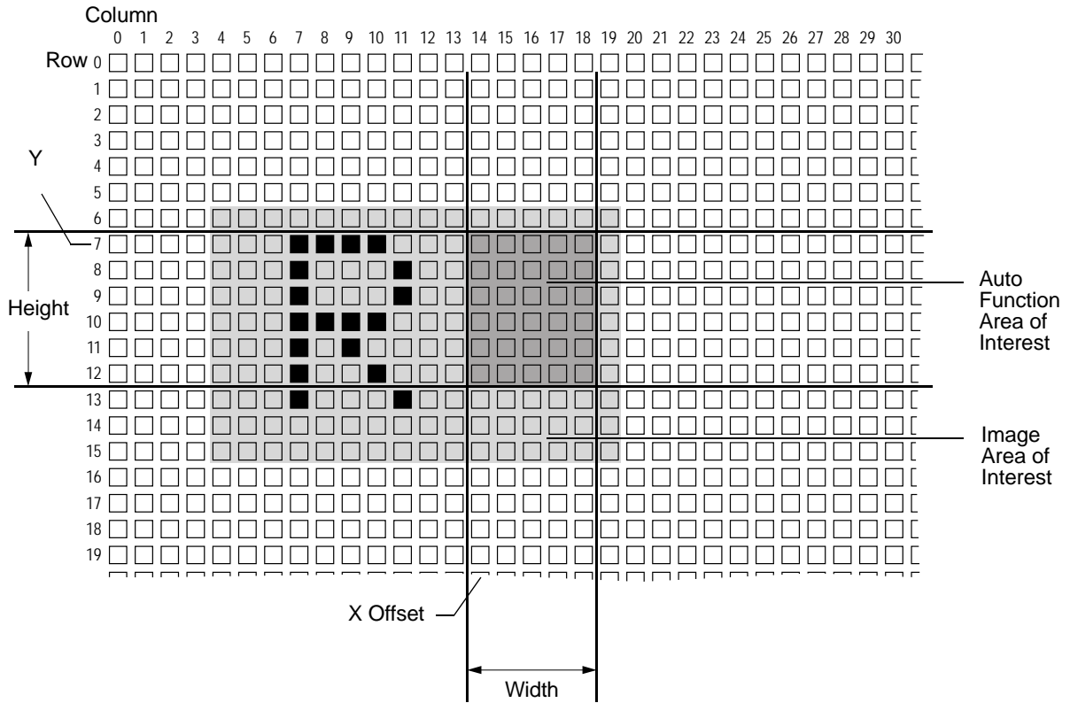
Fig. 117: Auto Function Area of Interest and Image Area of Interest
