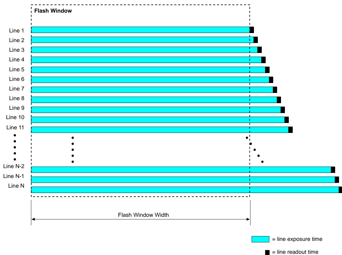
Fig. 65: Flash Window for Rolling Shutter in the Global Reset Release Mode
