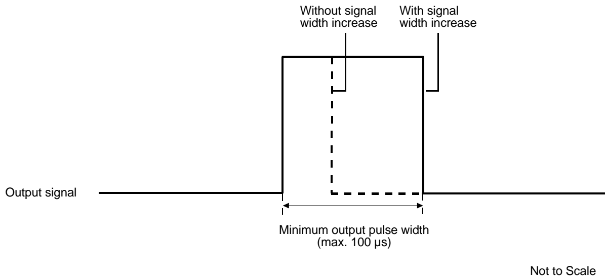
Fig. 119: Increasing the Signal Width of an Output Signal
