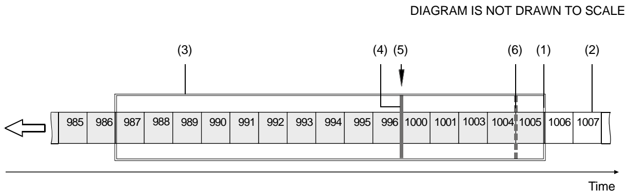
Fig. 125: Example of a Receive Window with Resend Request Threshold & Resend Request Batching Threshold
