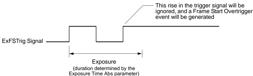
Fig. 53: Overtriggering with Timed Exposure
