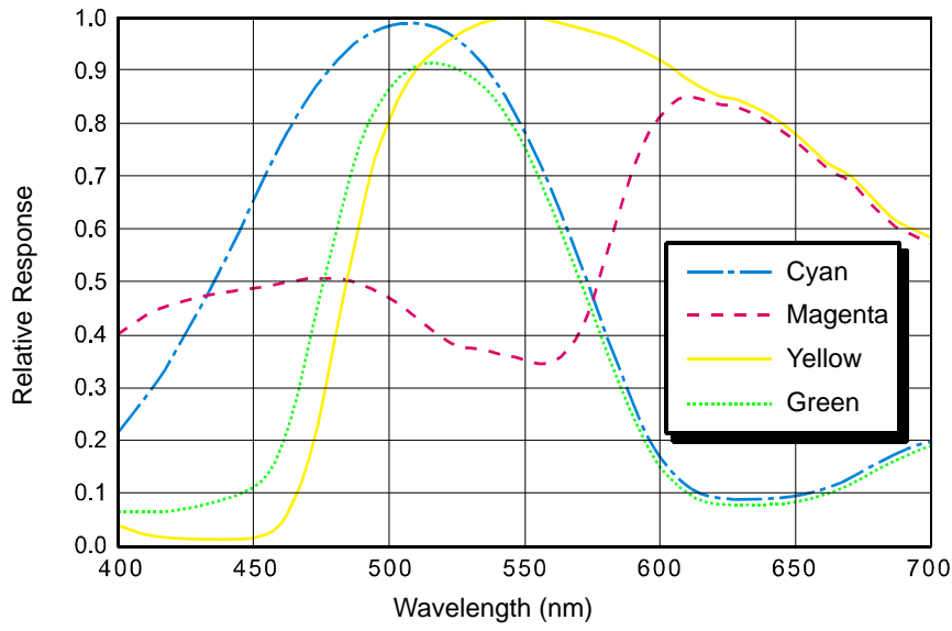
Fig. 17: acA750-30gc Spectral Response (From Sensor Data Sheet)
