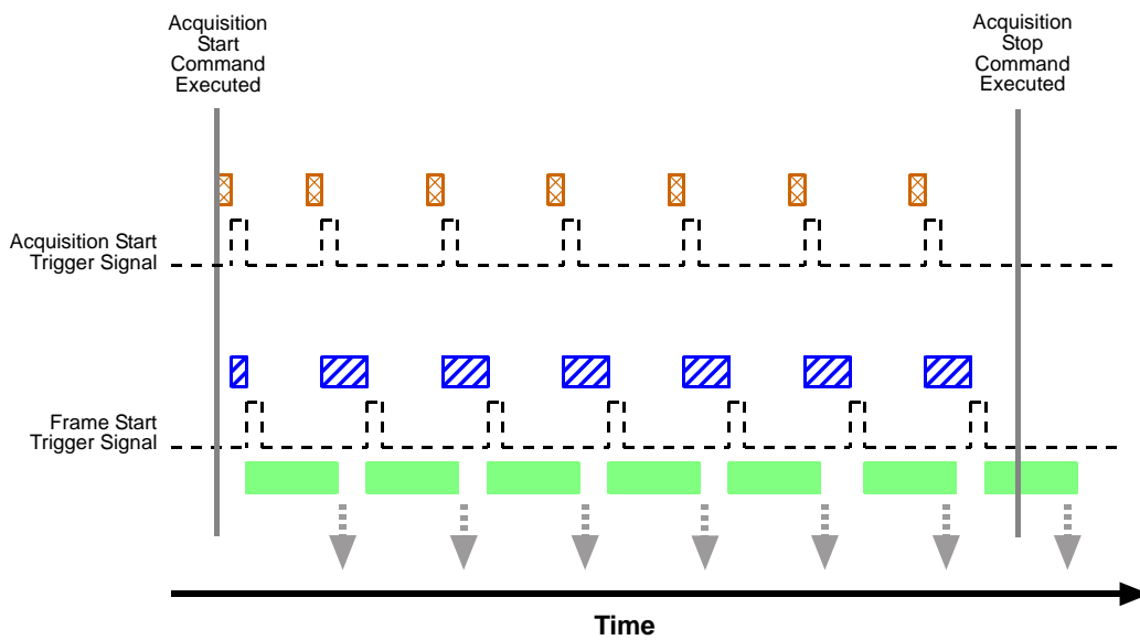
Fig. 82: Use Case 1 - Acquisition Start Trigger Off and Frame Start Trigger Off
