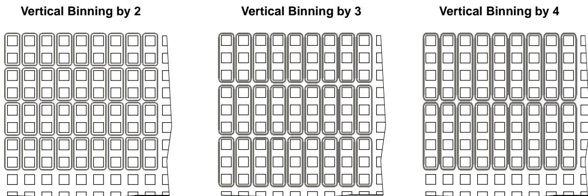
Fig. 103: Vertical Binning on Monochrome Cameras
