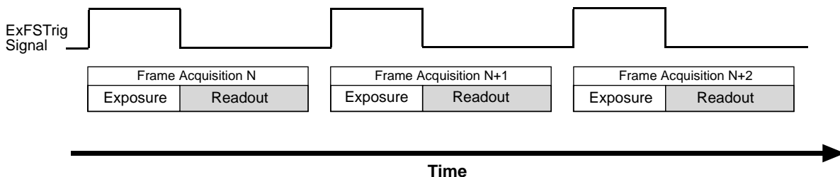
Fig. 67: Non-overlapped Exposure and Readout
