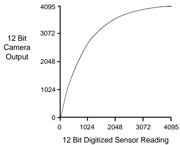
Fig. 116: Lookup Table with Values Mapped for Higher Camera Output at Low Sensor Readings
