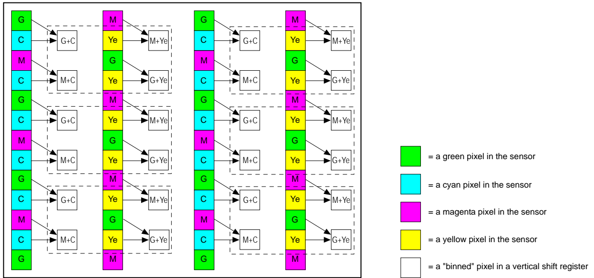
Fig. 88: Color Combinations for Field 0
