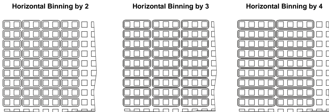
Fig. 104: Horizontal Binning on Monochrome Cameras
