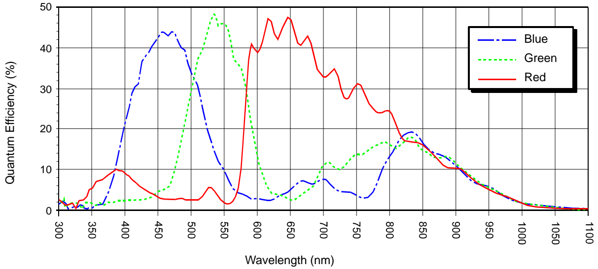
Fig. 23: acA2000-50gc, acA2000-50gc- CMV2000-V3, acA2040-25gc, acA2040-25gc- CMV4000-V3, Spectral Response (From Sensor Data Sheet)
