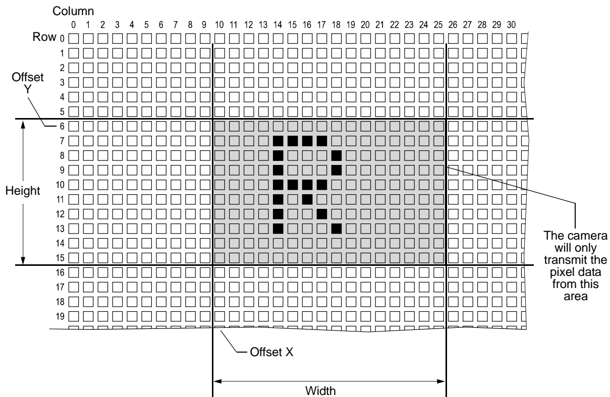
Fig. 94: Area of Interest
