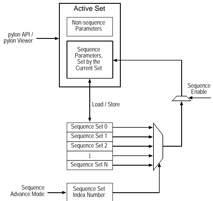
Fig. 96: Sequence Feature Block Diagram
