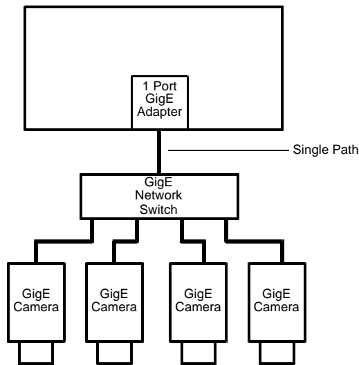
Fig. 128: Multiple Cameras on a Network
