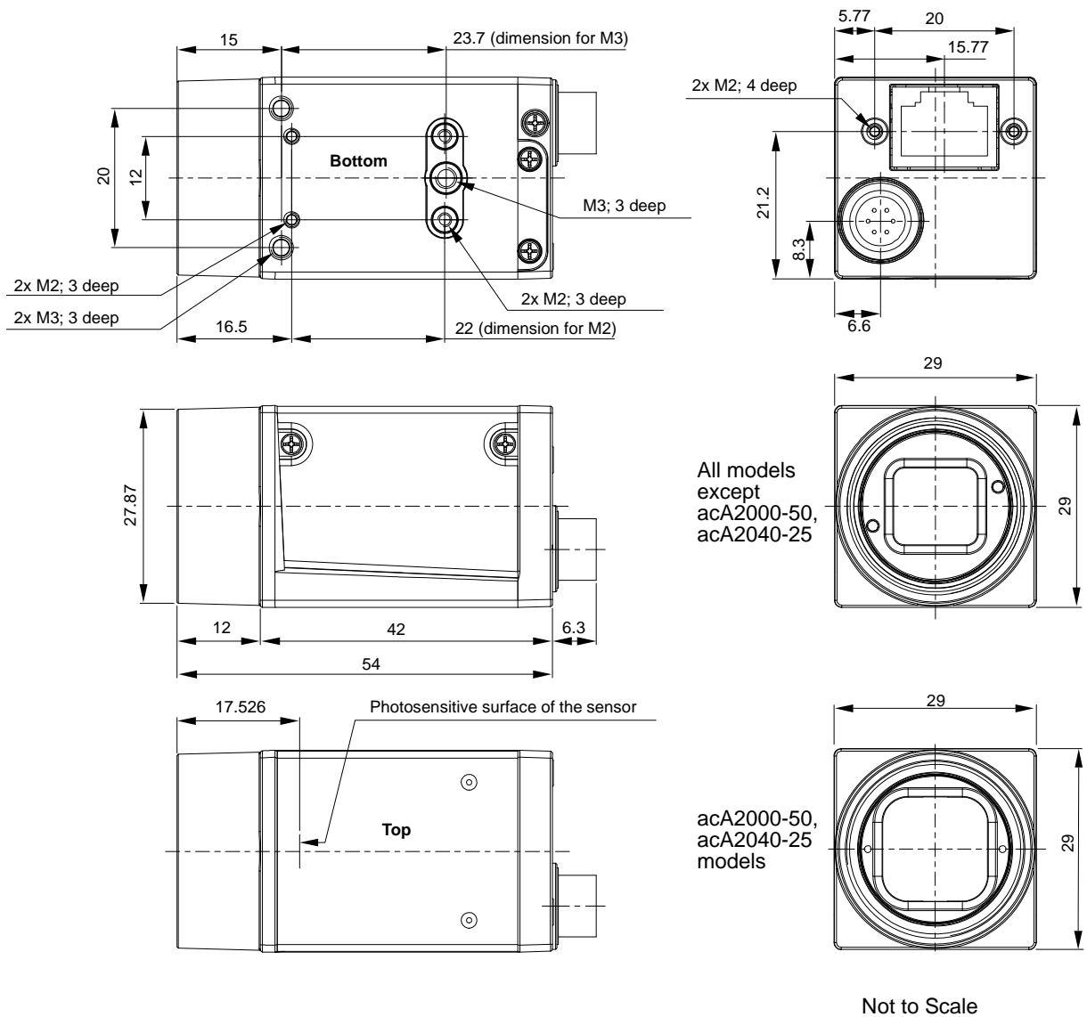
Fig. 25: Mechanical Dimensions (in mm) for Cameras with the C-mount Lens Adapter
