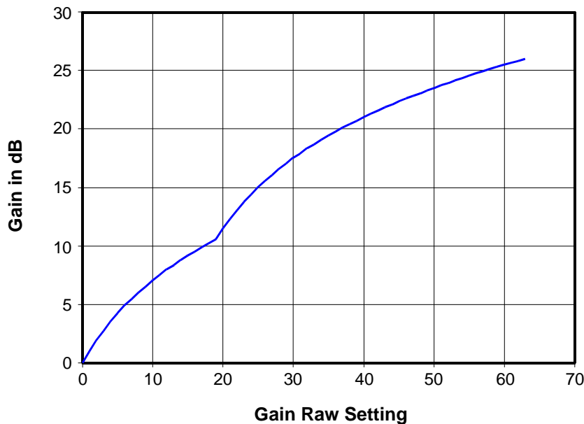
Fig. 93: Gain in dB Yielded by Gain Raw Settings
