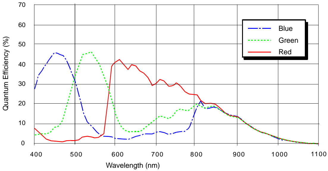
Fig. 19: acA1280-60gc, acA1300-60gc Spectral Response (From Sensor Data Sheet)
