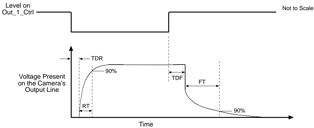
Fig. 45: Output Line Response Times
