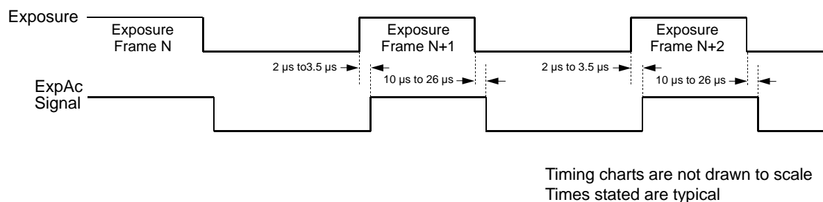
Fig. 73: Exposure Active Signal on Cameras with a Global shutter
