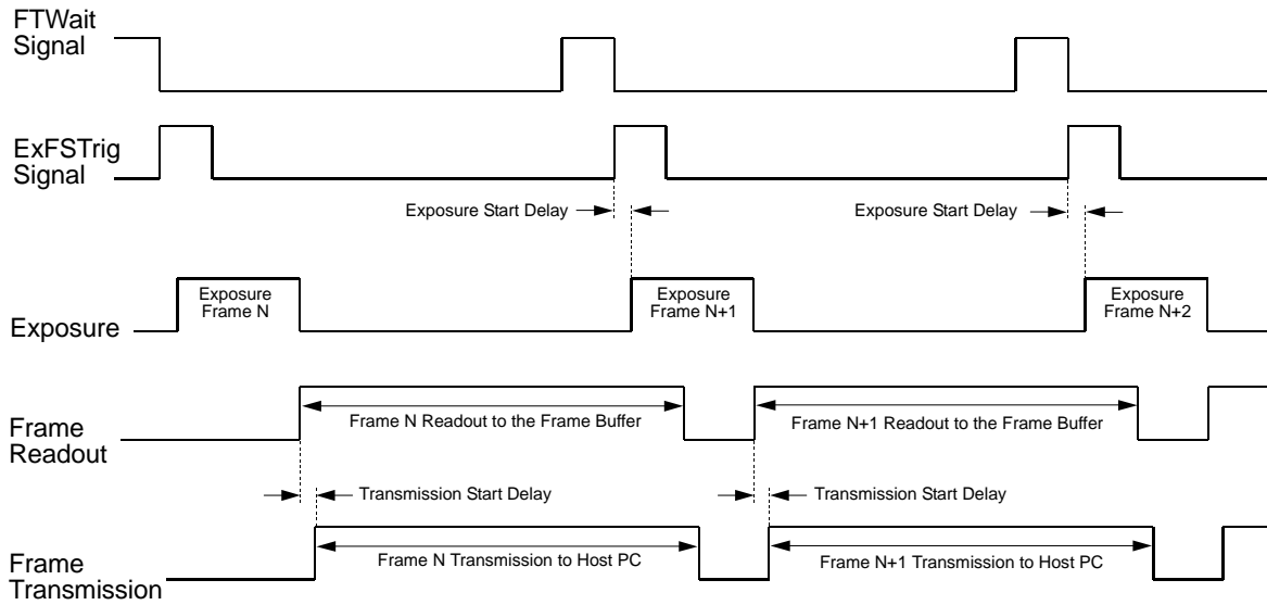
Fig. 81: Exposure Start Controlled with an ExFSTrig Signal
