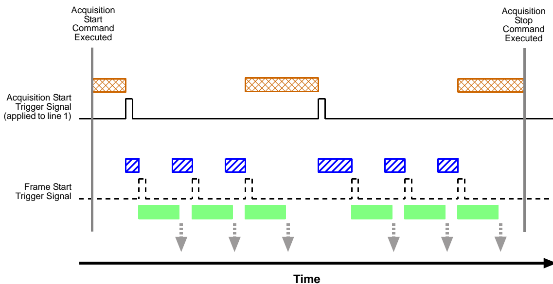
Fig. 84: Use Case 3 - Acquisition Start Trigger On and Frame Start Trigger Off
