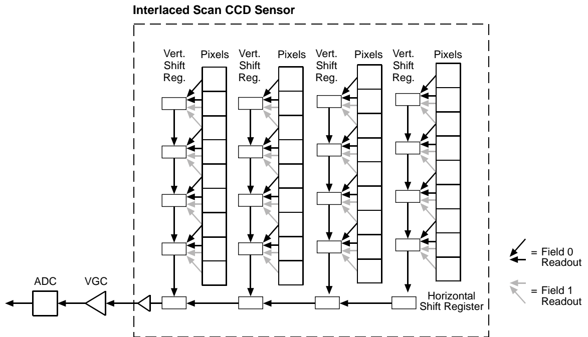
Fig. 30: CCD Sensor Architecture - Interlaced Scan Sensors
