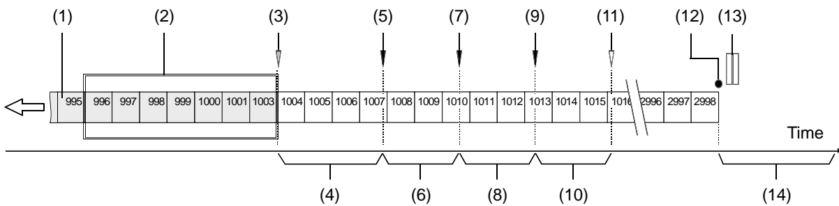
Fig. 126: Incomplete Stream of Packets and Part of the Resend Mechanism
