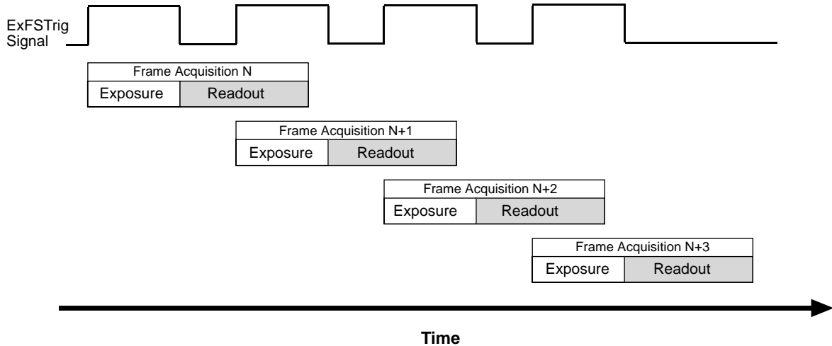
Fig. 68: Overlapped Exposure and Readout
