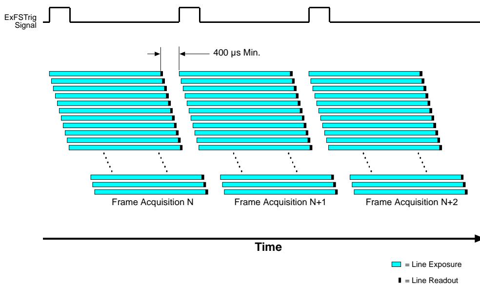
Fig. 72: Acquisition Overlap Guideline
