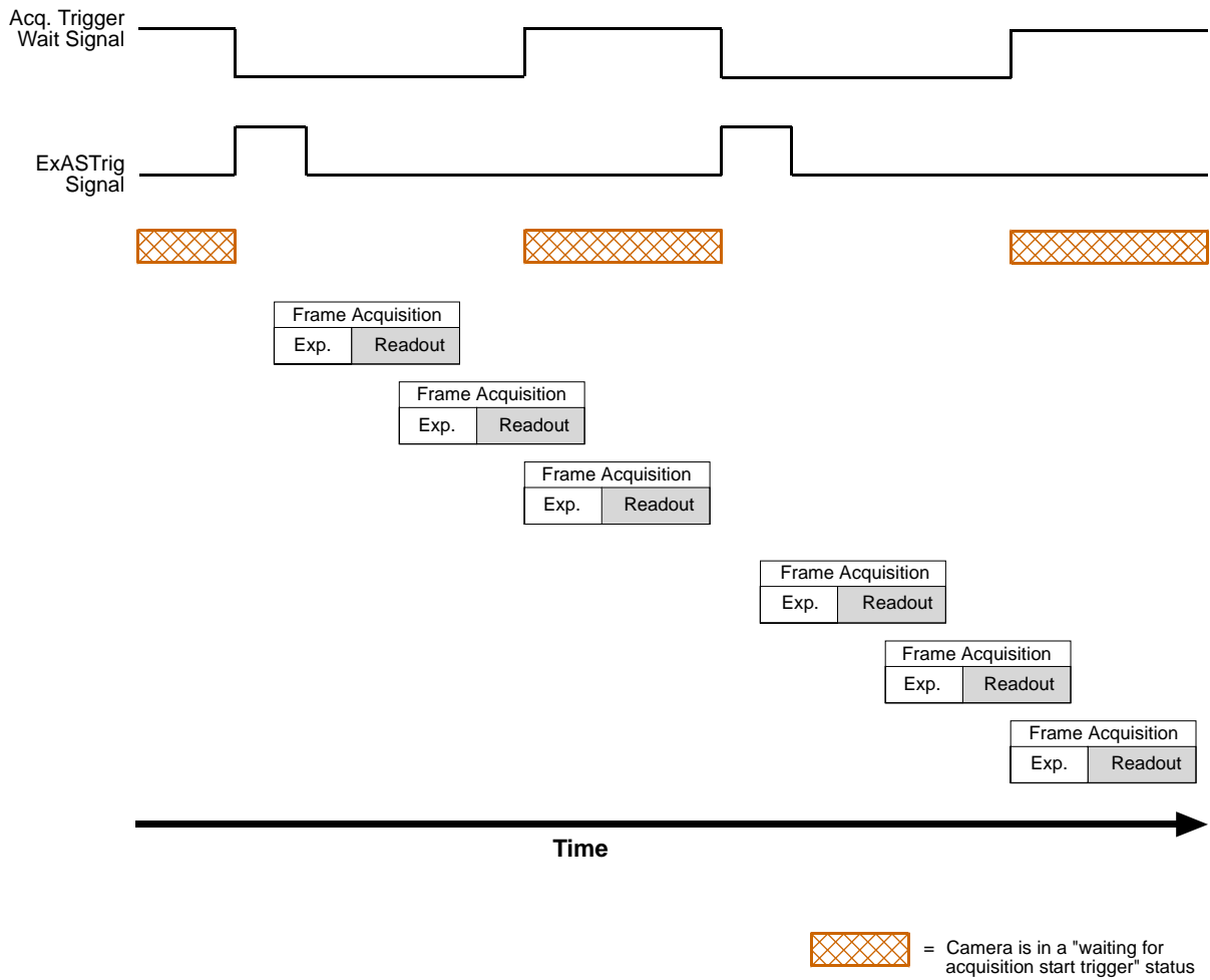
Fig. 76: Acquisition Trigger Wait Signal
