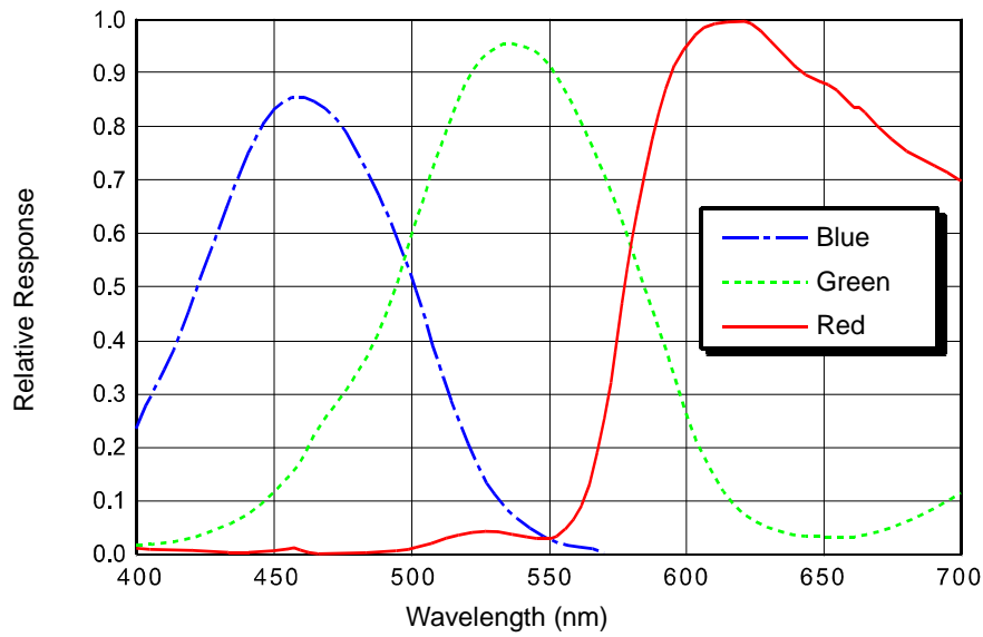
Fig. 21: acA1600-20gc Spectral Response (From Sensor Data Sheet)
