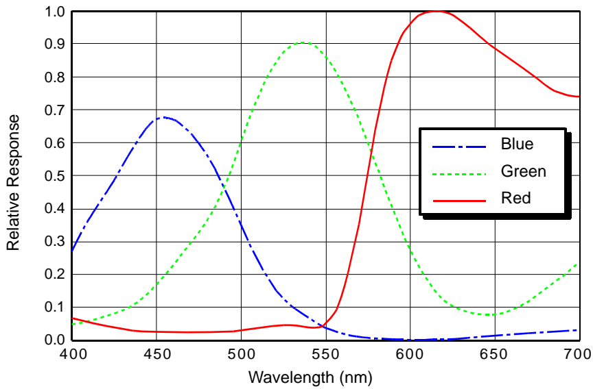
Fig. 20: acA1300-22gc, acA1300-30gc Spectral Response (From Sensor Data Sheet)
