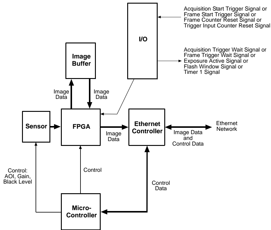
Fig. 35: Camera Block Diagram
