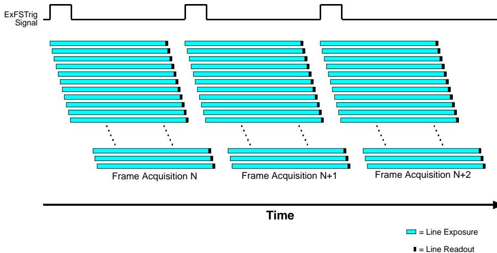
Fig. 71: Overlapped Exposure and Readout
