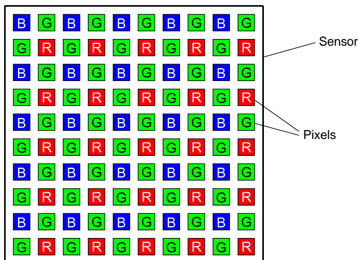
Fig. 86: Bayer Filter Pattern
