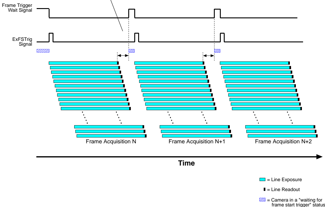
Fig. 80: Frame Trigger Wait Signal on a Rolling Shutter Camera
