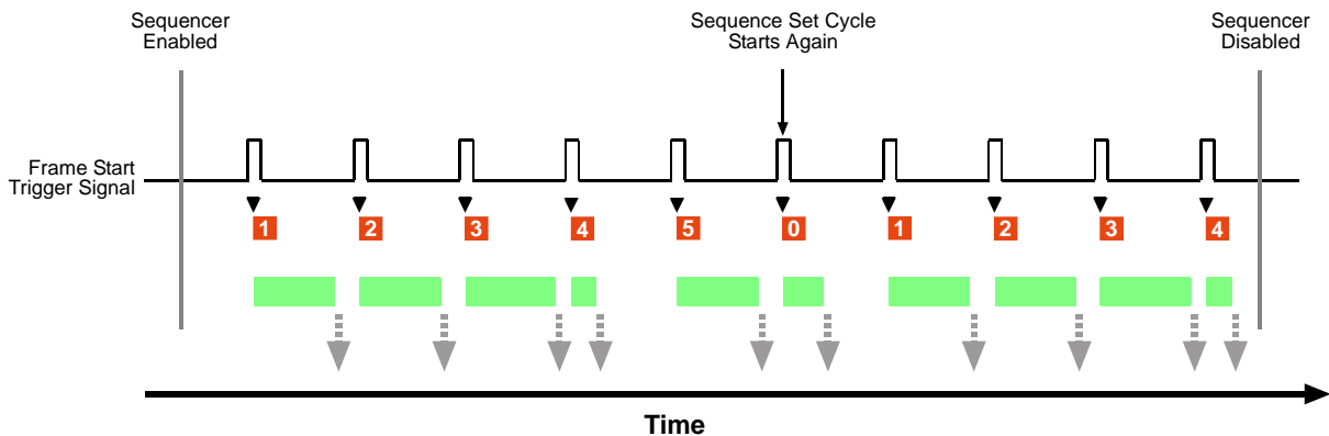
Fig. 98: Sequencer in Controlled Sequence Advance Mode with Always Active as the Sequence Control Source
