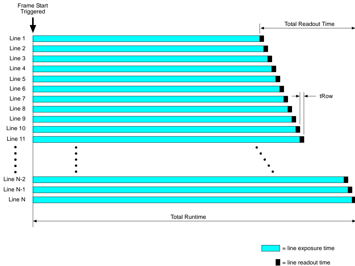
Fig. 63: Rolling Shutter in the Global Reset Release Mode
