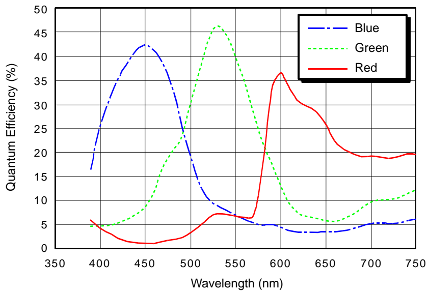
Fig. 24: acA1920-25gc, acA2500-14gc, Spectral Response (From Sensor Data Sheet)
