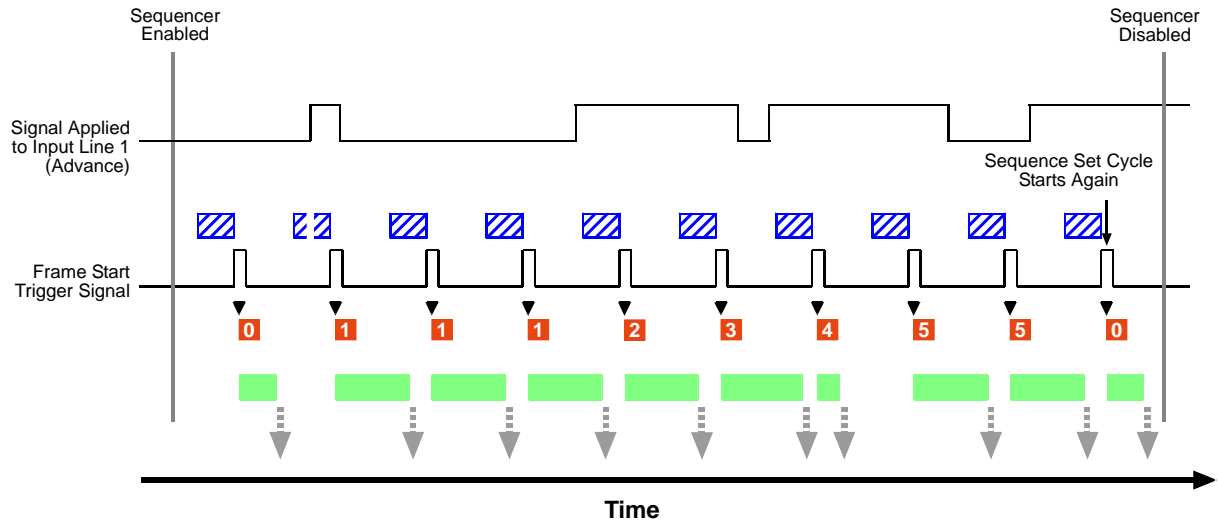
Fig. 100: Sequencer in Controlled Sequence Advance Mode with Line 1 as the Sequence Control Source
