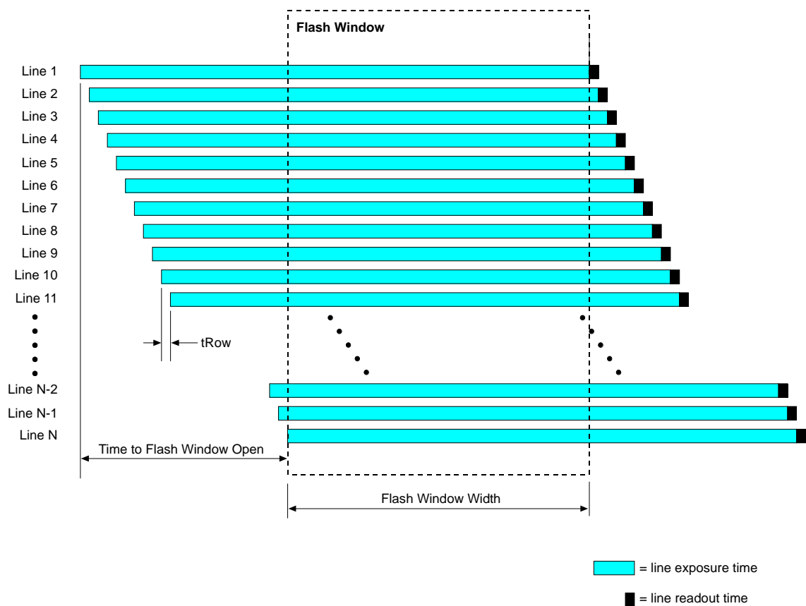
Fig. 64: Flash Window for Rolling Shutter in the ERS Mode
