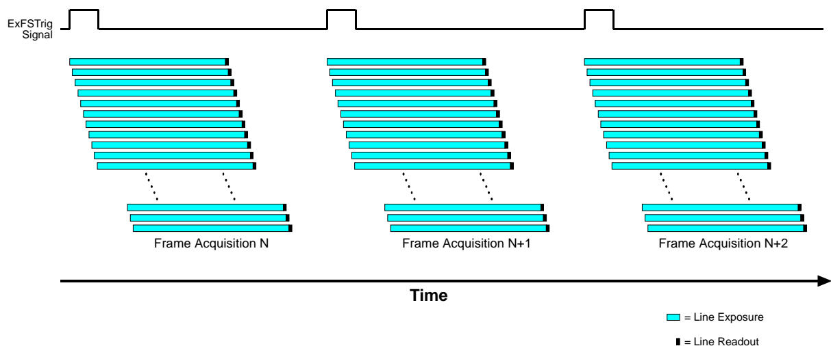
Fig. 70: Non-overlapped Acquisition
