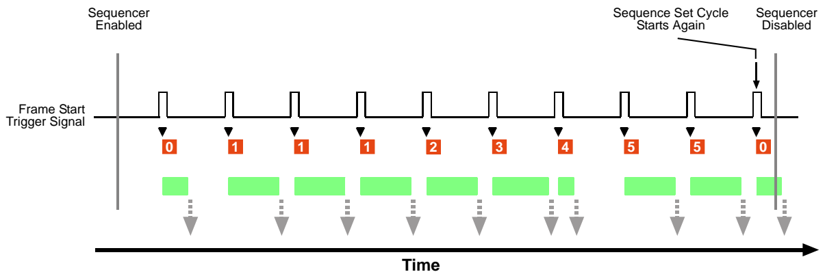
Fig. 97: Sequencer in Auto Sequence Advance Mode
