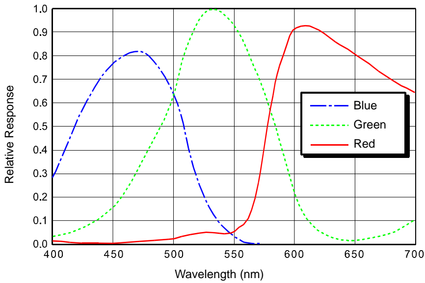
Fig. 16: acA645-100gc Spectral Response (From Sensor Data Sheet)
