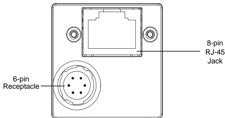
Fig. 36: Camera Connectors
