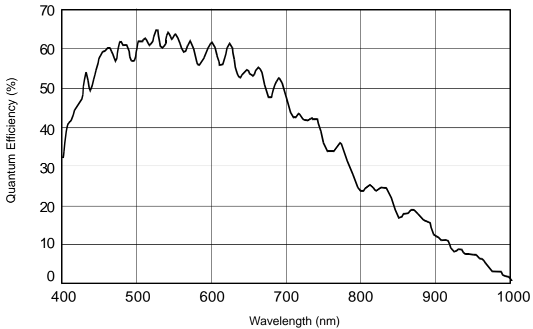
Fig. 11: acA2000-50gm, acA2000-50gm-CMV2000-V3, acA2040-25gm, acA2040-25gm-CMV4000-V3, Spectral Response (From Sensor Data Sheet)
