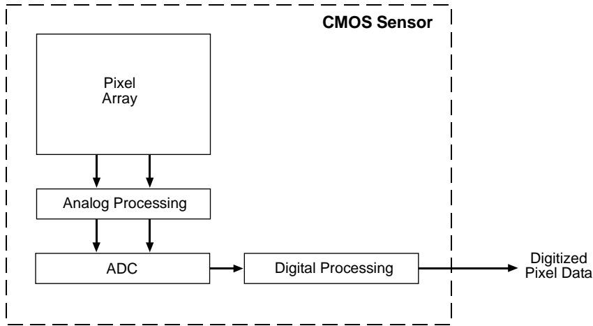
Fig. 32: CMOS Sensor Architecture
