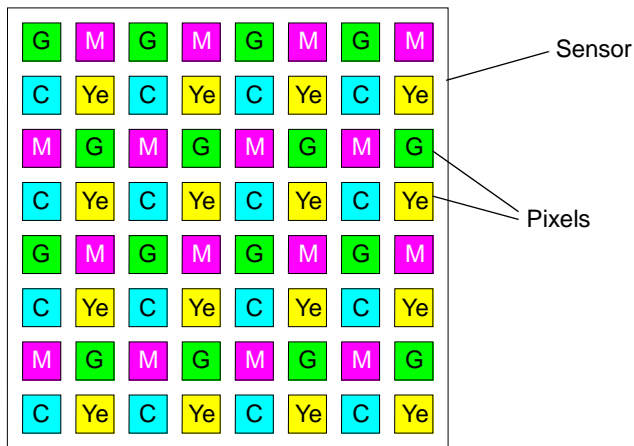
Fig. 87: Complementary Color Filter Pattern
