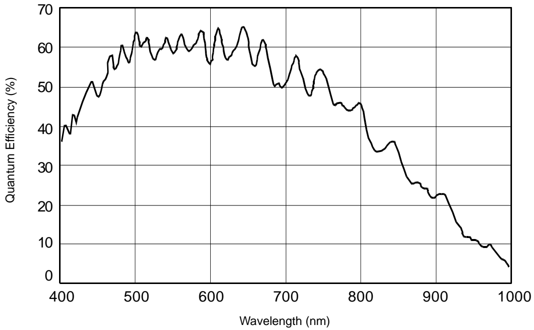
Fig. 12: acA2000-50gmNIR, acA2000-50gmNIR- CMV2000-V3,acA2040-25gmNIR, acA2040-25gmNIR- CMV4000-V3, Spectral Response (From Sensor Data Sheet) (*)
