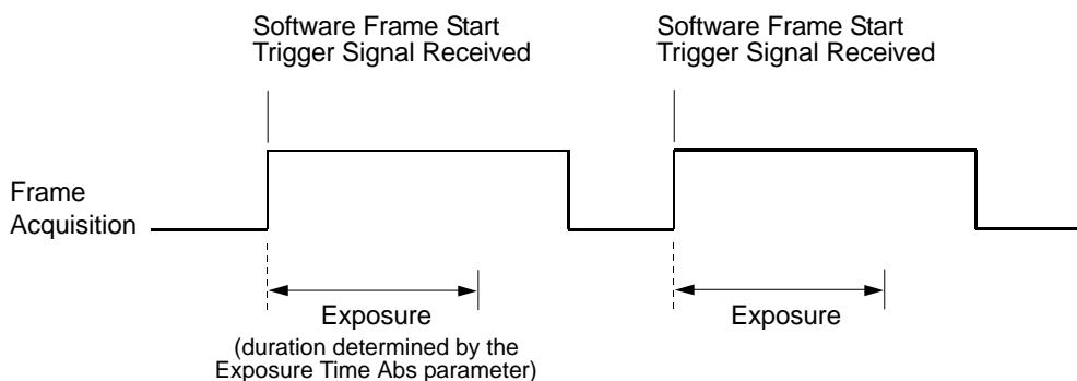
Fig. 51: Frame Acquisition with a Software Frame Start Trigger
