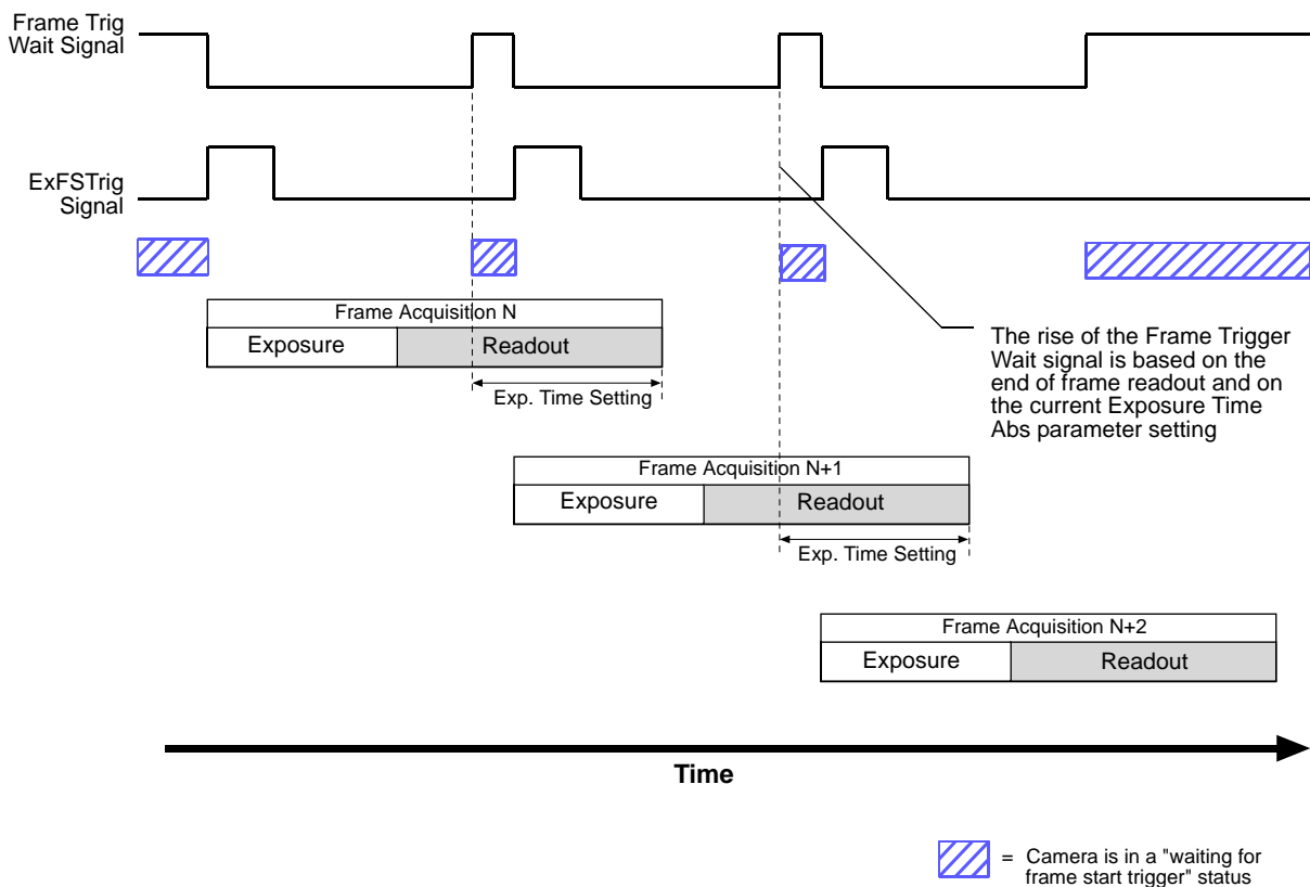
Fig. 78: Frame Trigger Wait Signal with the Timed Exposure Mode
