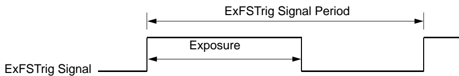
Fig. 54: Trigger Width Exposure with Rising Edge Triggering
