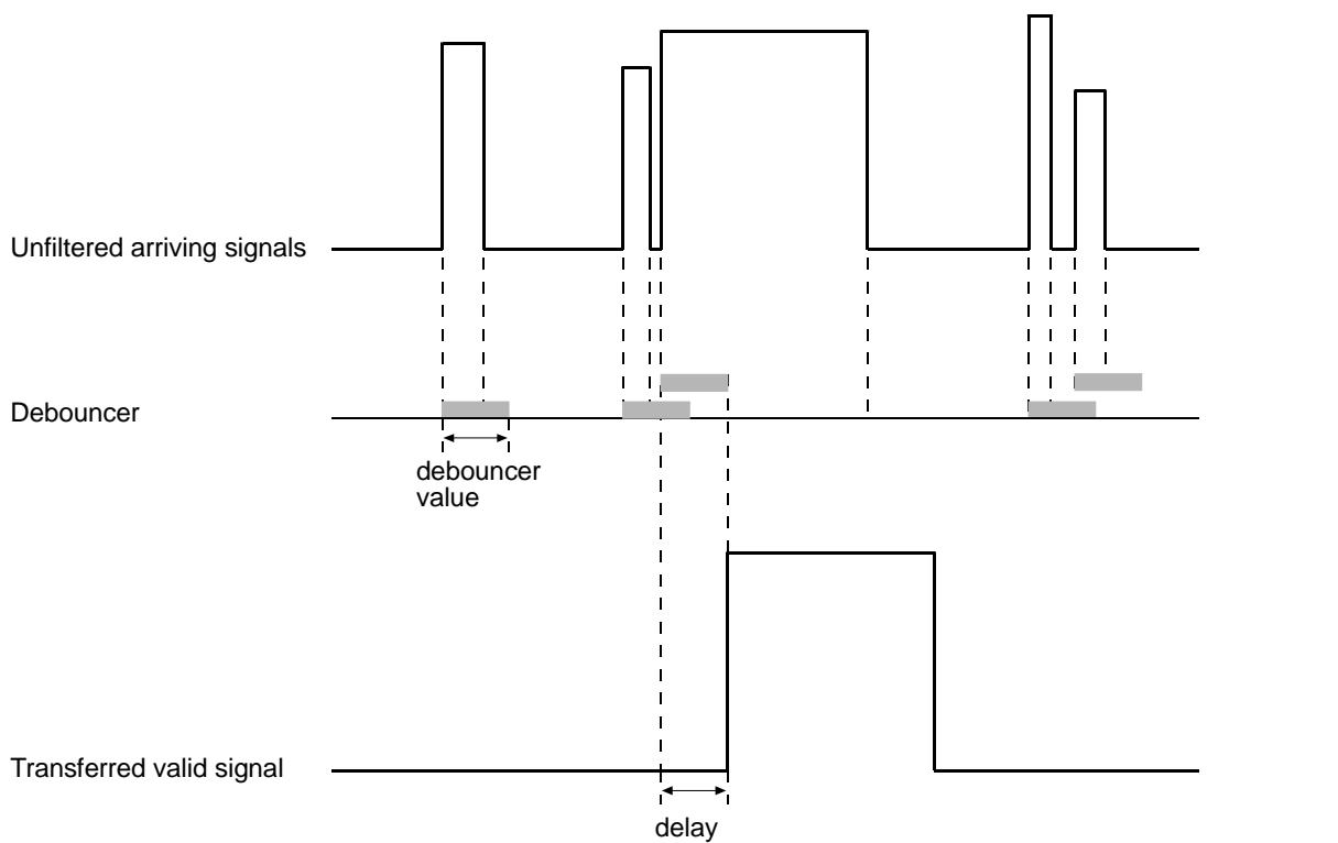
Fig. 46: Filtering of Input Signals by the Debouncer
