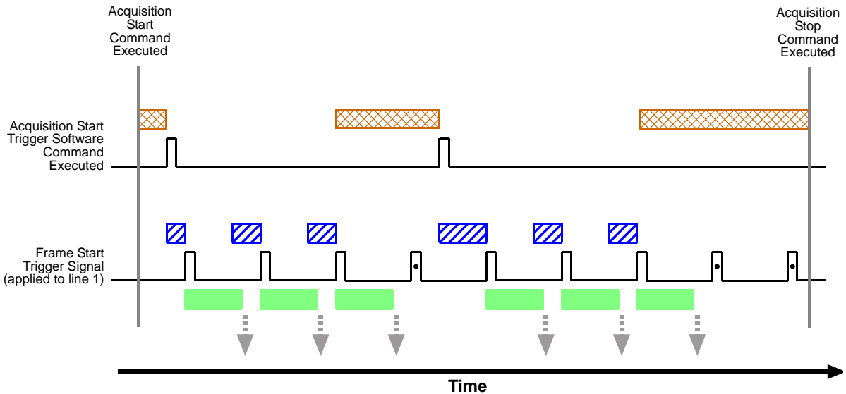
Fig. 85: Use Case 4 - Acquisition Start Trigger On and Frame Start Trigger On
