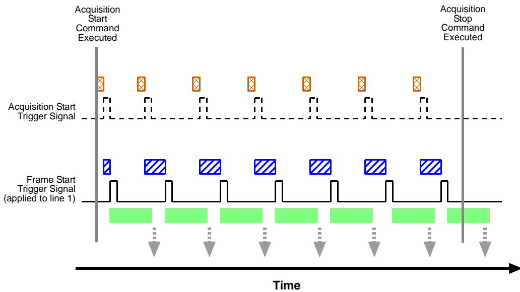
Fig. 83: Use Case 2 - Acquisition Start Trigger Off and Frame Start Trigger On
