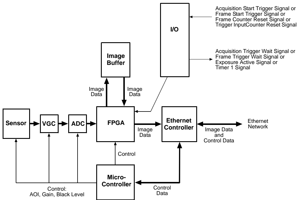
Fig. 31: Camera Block Diagram
