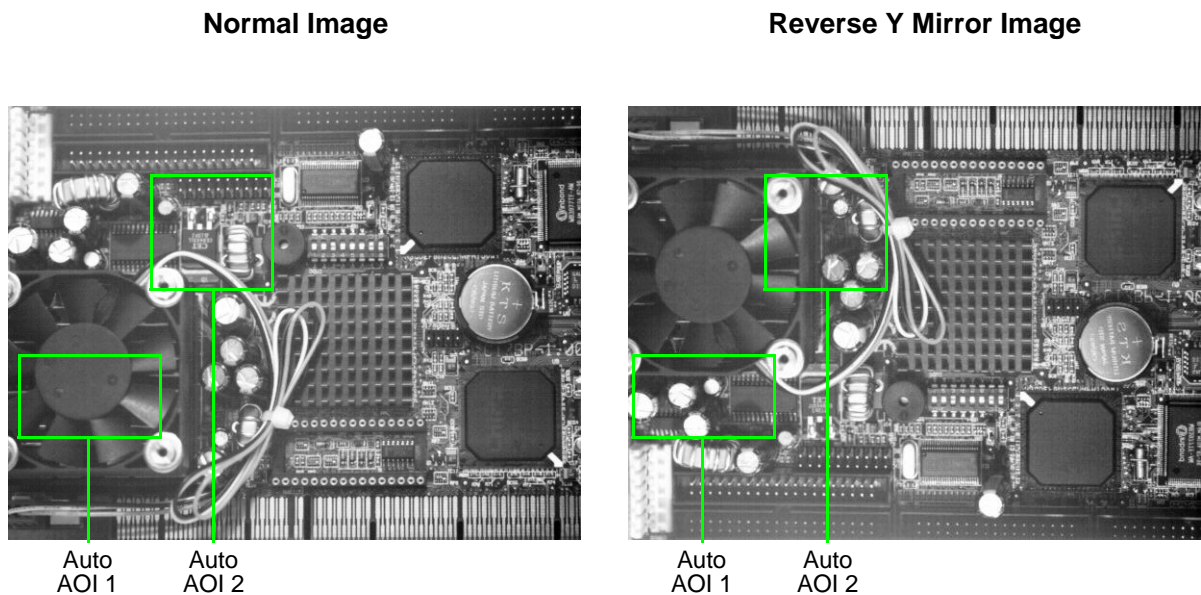
Fig. 114: Using Reverse Y Mirror Imaging with Auto Functions Enabled
