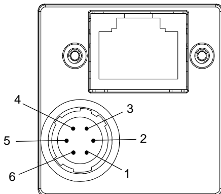
Fig. 37: Pin Numbering for the 6-pin Connector
