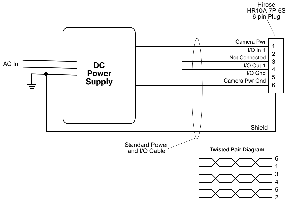
Fig. 38: Standard Power and I/O Cable
