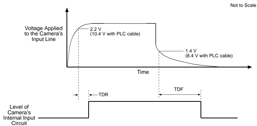
Fig. 41: Input Line Response Times
