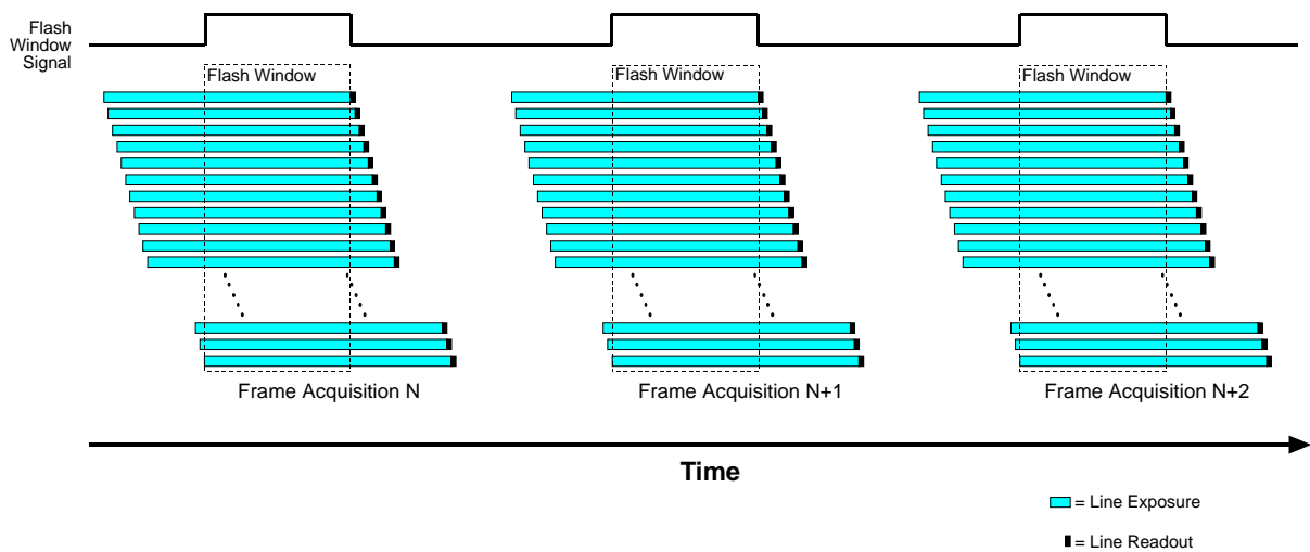
Fig. 75: Flash Window Signal on Cameras with a Rolling Shutter
