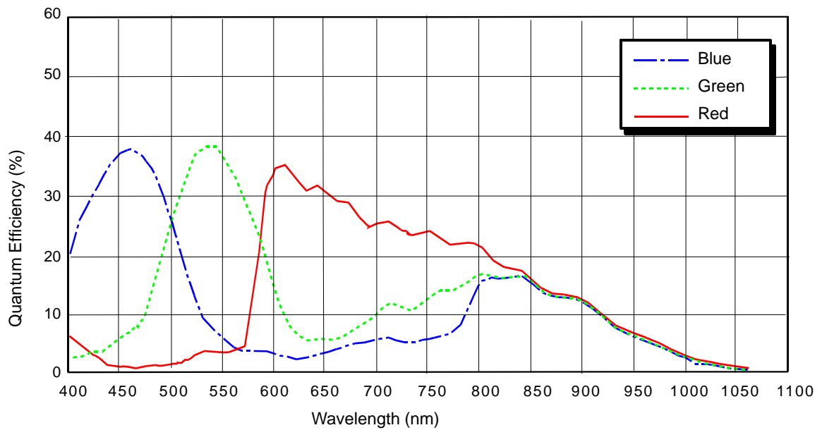
Fig. 22: acA1600-60gc Spectral Response (From Sensor Data Sheet)
