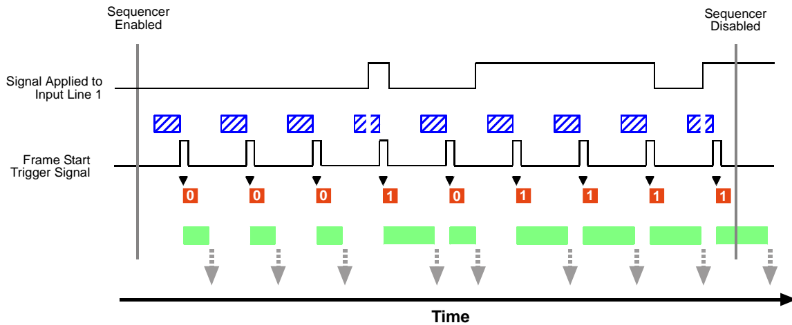
Fig. 102: Sequencer in Free Selection Mode
