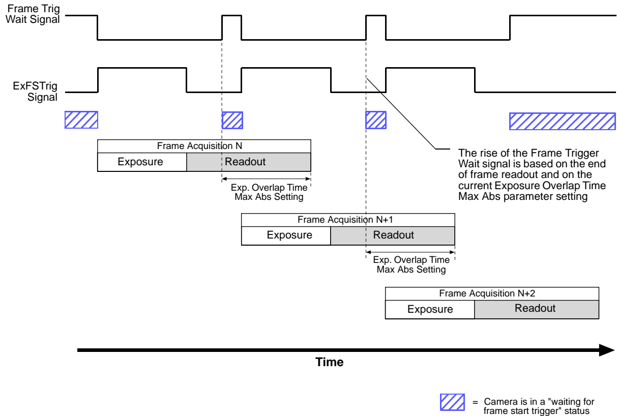
Fig. 79: Frame Trigger Wait Signal with the Trigger Width Exposure Mode
