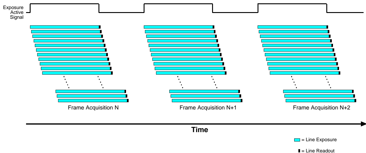
Fig. 74: Exposure Active Signal on Cameras with a Rolling shutter
