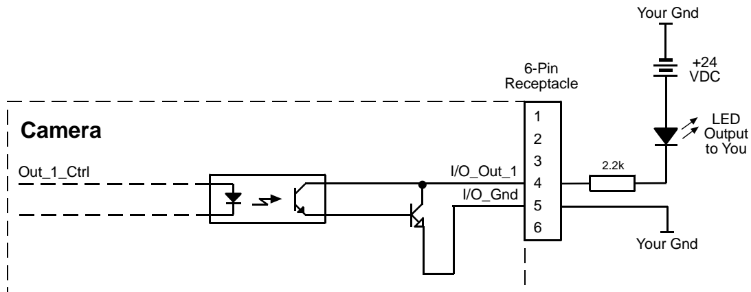
Fig. 44: Typical LED Output Signal at +24 VDC for the External Circuit (Simplified Example)
