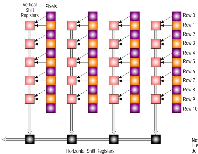
Fig. 55: Field 0 Readout
