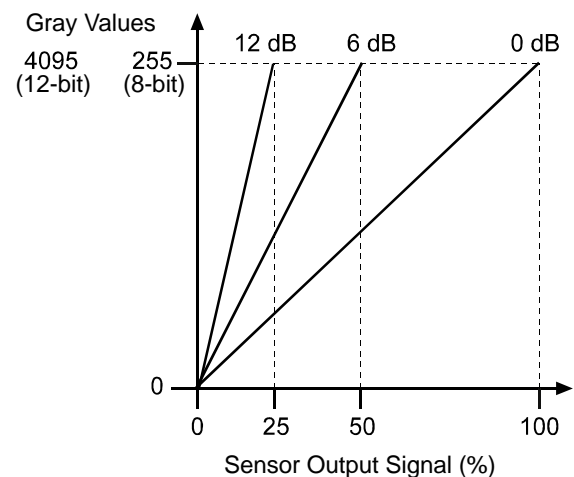
Fig. 92: Gain in dB
