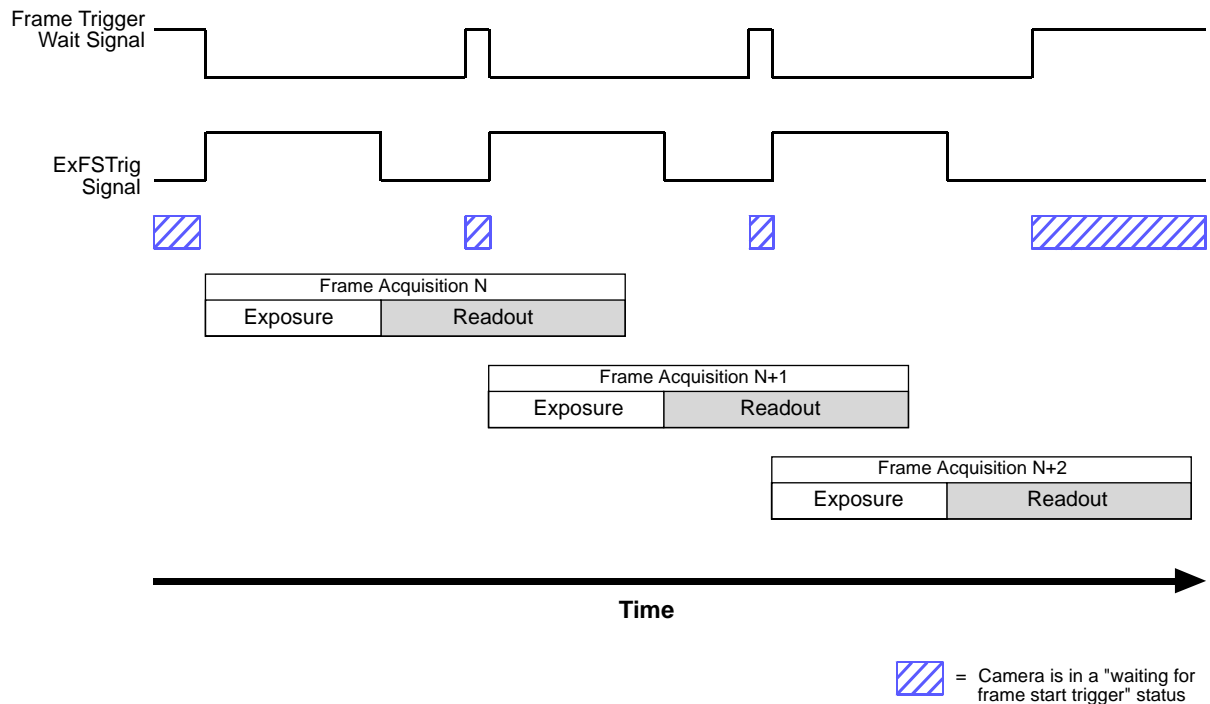
Fig. 77: Frame Trigger Wait Signal
