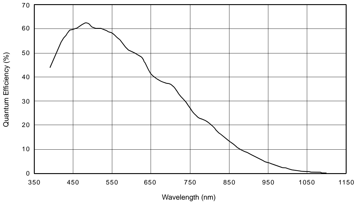
Fig. 13: acA2500-14gm, acA1920-25gm Spectral Response (From Sensor Data Sheet)
