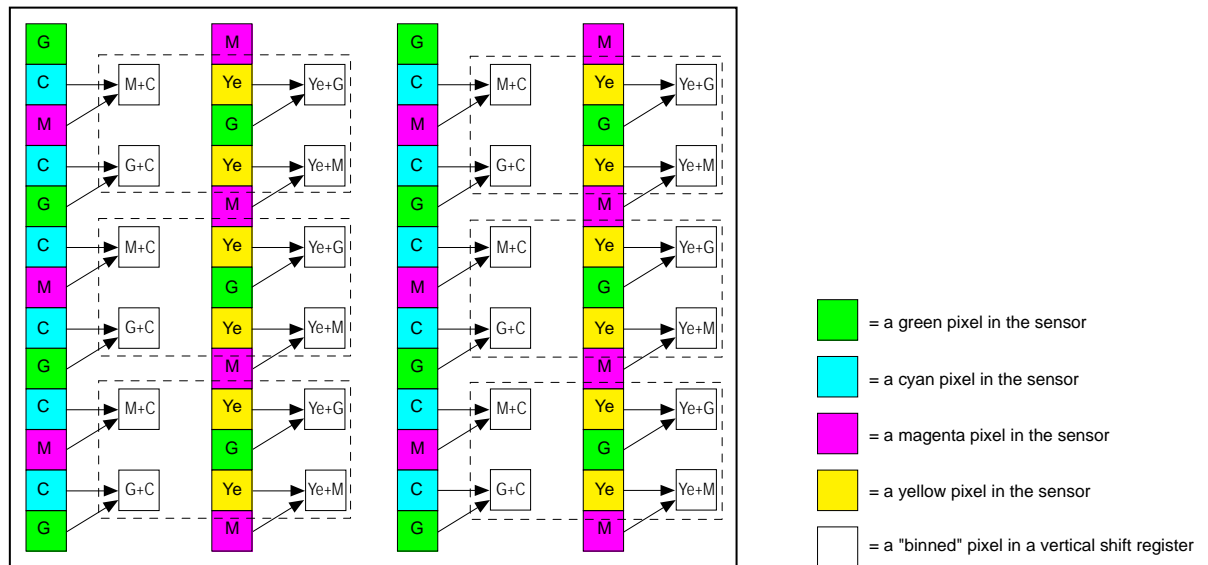
Fig. 89: Color Combinations for Field 1
