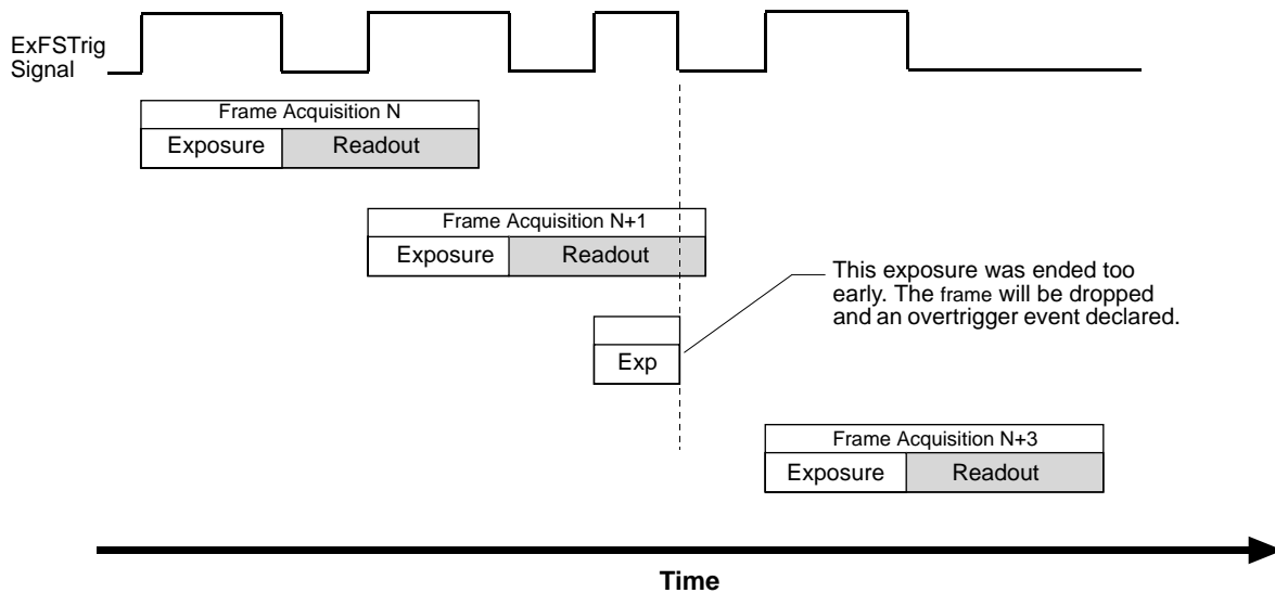
Fig. 69: Overtriggering Caused by an Early End of Exposure
