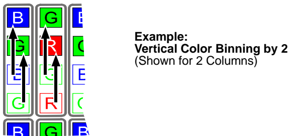
Fig. 105: Vertical Color Binning by 2
