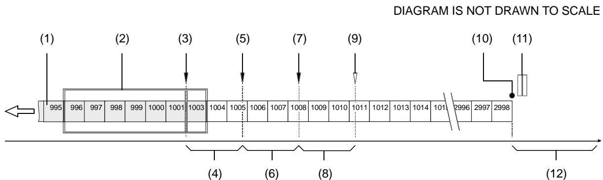
Fig. 127: Combination of Threshold Resend Mechanism and Timeout Resend Mechanism
