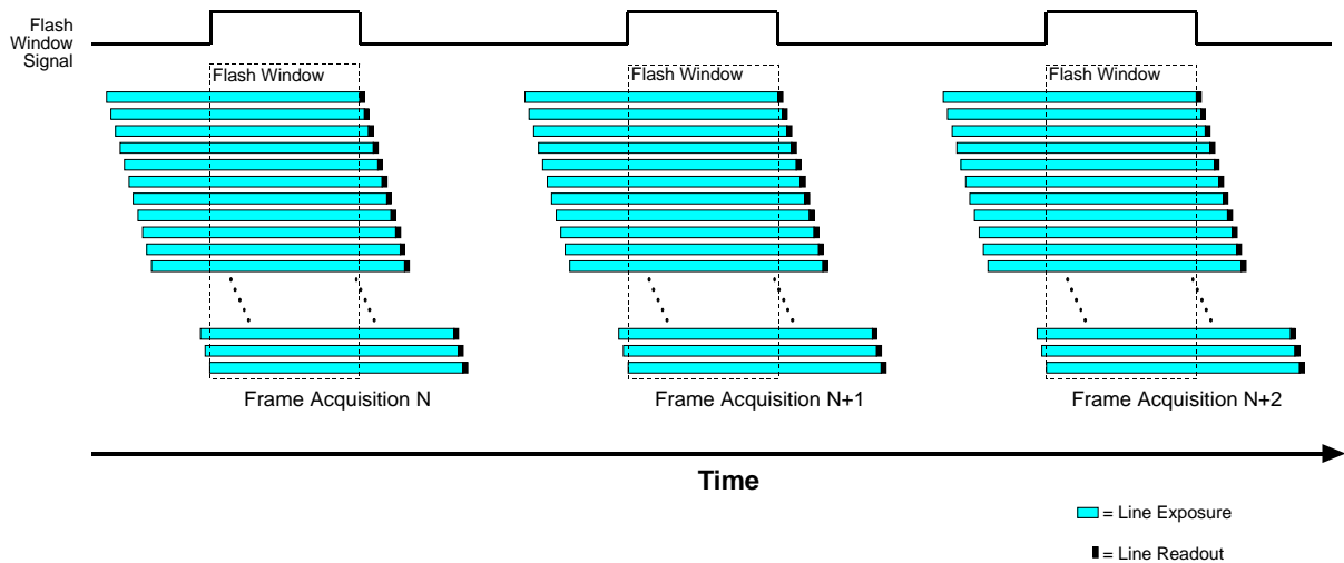
Fig. 66: Flash Window Signal on Cameras with a Rolling Shutter
