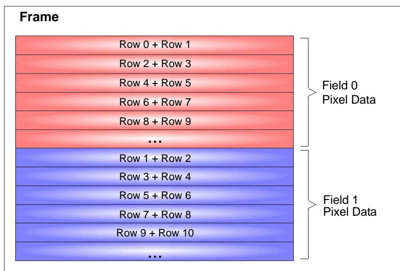
Fig. 59: Concatenated New Fields Output Mode
