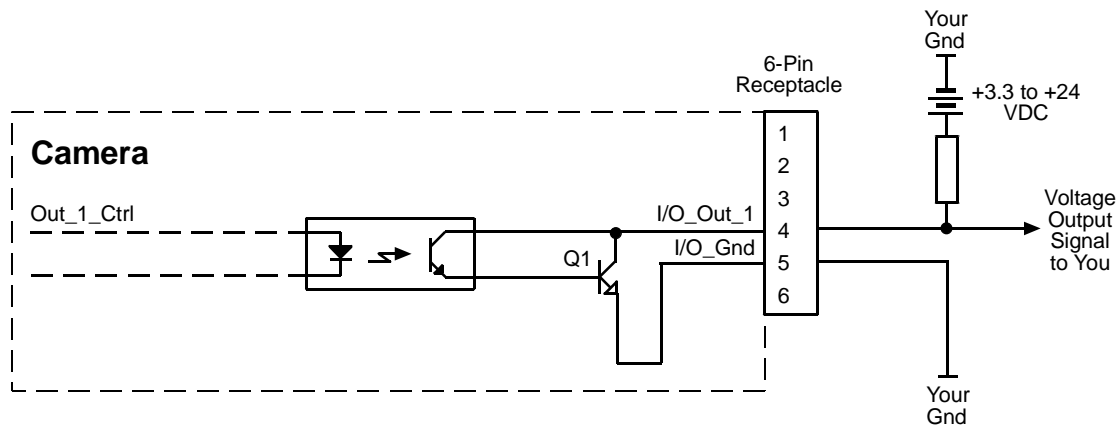
Fig. 43: Typical Voltage Output Circuit (Simplified Example)
