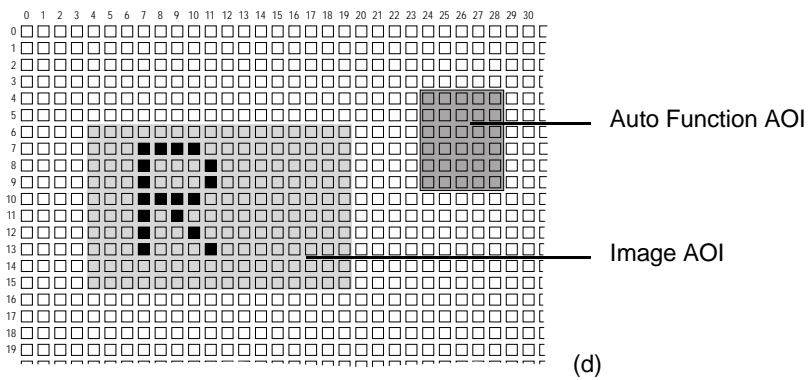
Fig. 118: Various Degrees of Overlap Between the Auto Function AOI and the Image AOI
