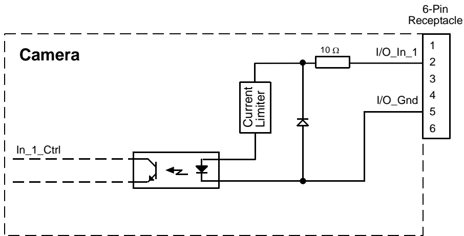
Fig. 39: Input Line Schematic (Simplified)
