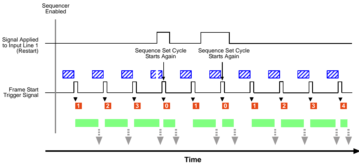
Fig. 99: Sequencer in Controlled Sequence Advance Mode with Always Active as the Sequence Control Source and Synchronous Restart Controlled by Line 1
