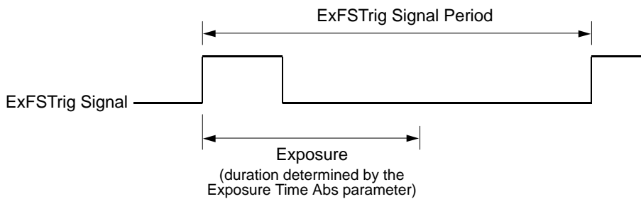
Fig. 52: Timed Exposure with Rising Edge Triggering
