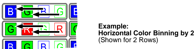
Fig. 106: Horizontal Color Binning by 2
