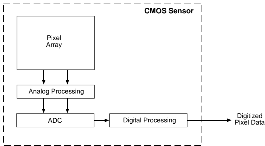
Fig. 34: CMOS Sensor Architecture
