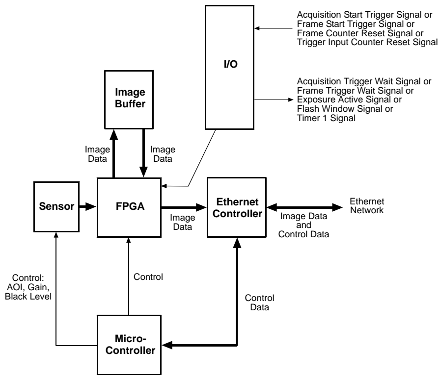
Fig. 33: Camera Block Diagram
