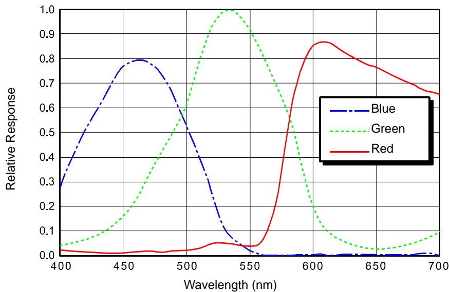
Fig. 14: acA640-90gc Spectral Response (From Sensor Data Sheet)
