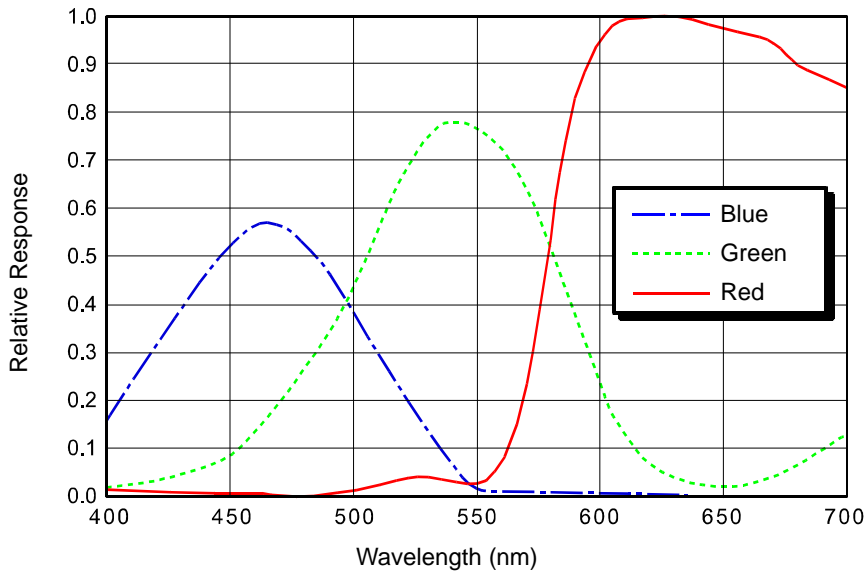
Fig. 15: acA640-120gc Spectral Response (From Sensor Data Sheet)
