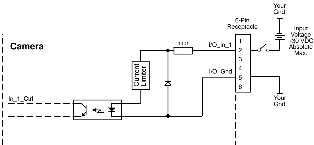
Fig. 40: Typical Input Circuit (Simplified)
