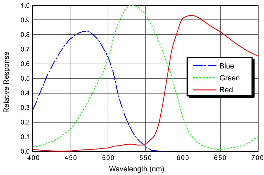
Fig. 18: acA780-75gc Spectral Response (From Sensor Data Sheet)
